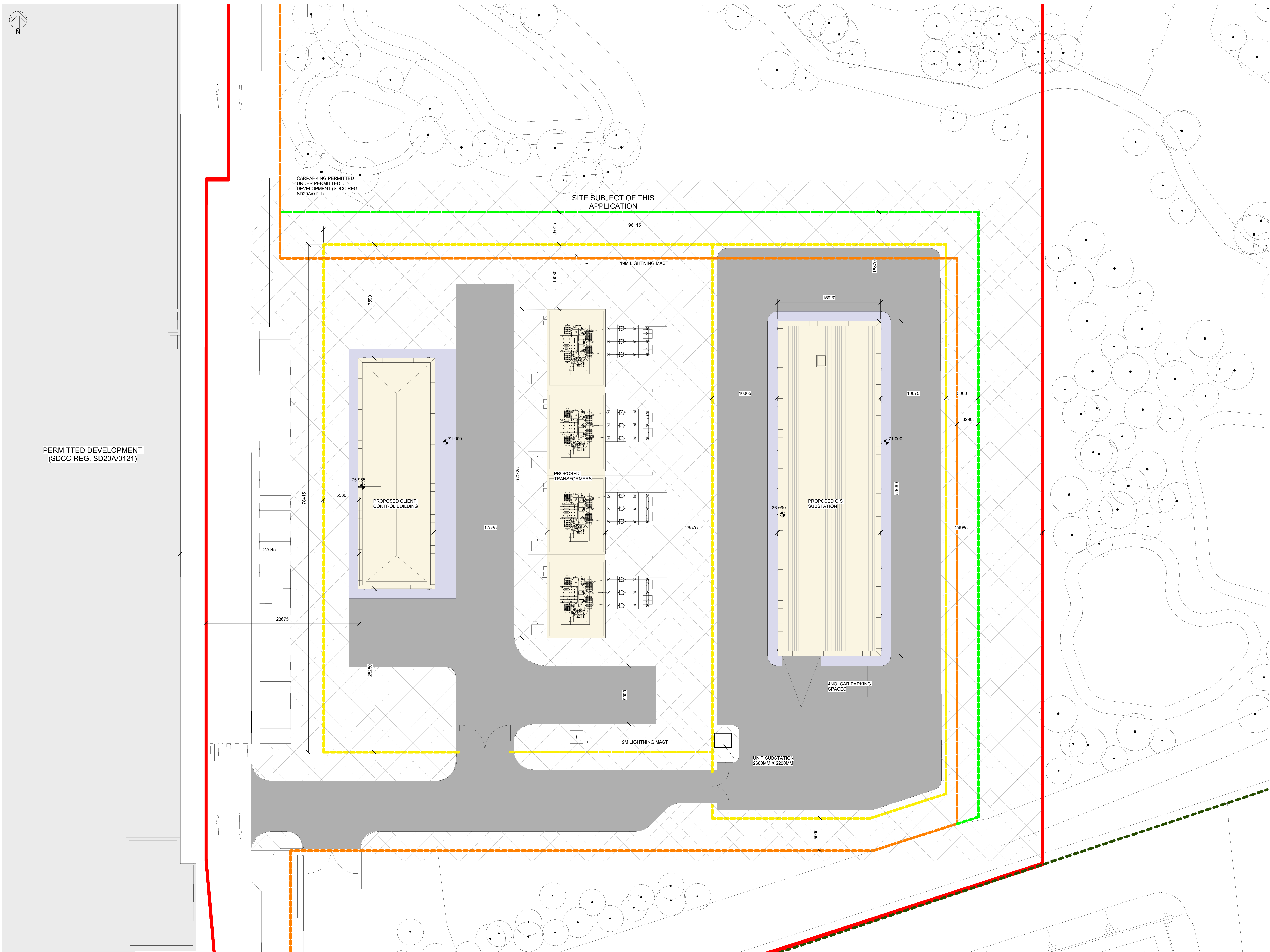
1 PROPOSED BUILDINGS & ROAD PLAN 1 : 200
